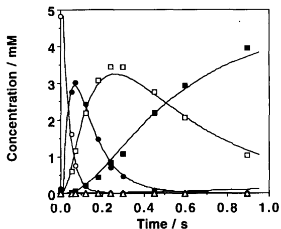
Fig. 3. Reaction curves for ATP hydrolysis using preheater. The reaction was performed in aqueous solution containing 0.005 M ATP, 0.1 M NaCl, 0.05 M MgCl 2 , 0.05 M imidazole (initial pH at 25 °C = 7.0) with 38 cm tubing in main heater and 38 cm tubing in preheater which is heated at 200 °C, 14 MPa. ○, ATP; ●, ADP; □, AMP; ■, adenosine; △, adenine. The line drawn through the experimental points were fitted by SIMFIT.
